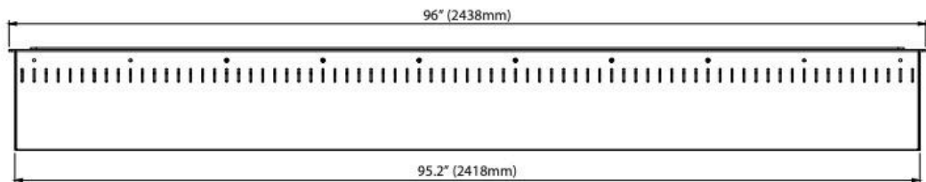
FRONT VIEW
