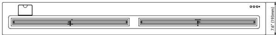
TOP VIEW
